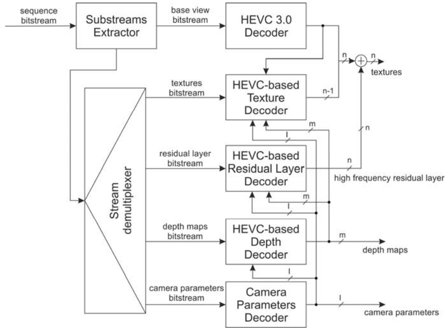
Fig. 2. Scheme of the described decoder.
